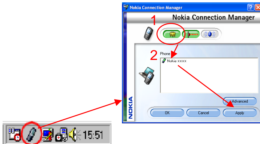
Figure 1. Double click on the Nokia Connection Manager icon open the Nokia Connection Manager. Now connect your phone to PC and select the same connection method in Nokia Connection Manager as you used for connecting your phone (Step 1). Now you should see your phone listed, select your phone (Step 2) and click Apply (Step 3).
